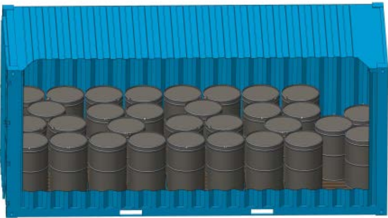
Figure 6—MPF ISO Loaded with 55-Gallon DOT 7A Type A or UN1A2 Drums
