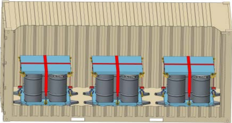
Figure 5—MPF ISO Loaded with 9975 Shipping Packages in Cargo Restraint Transporters
