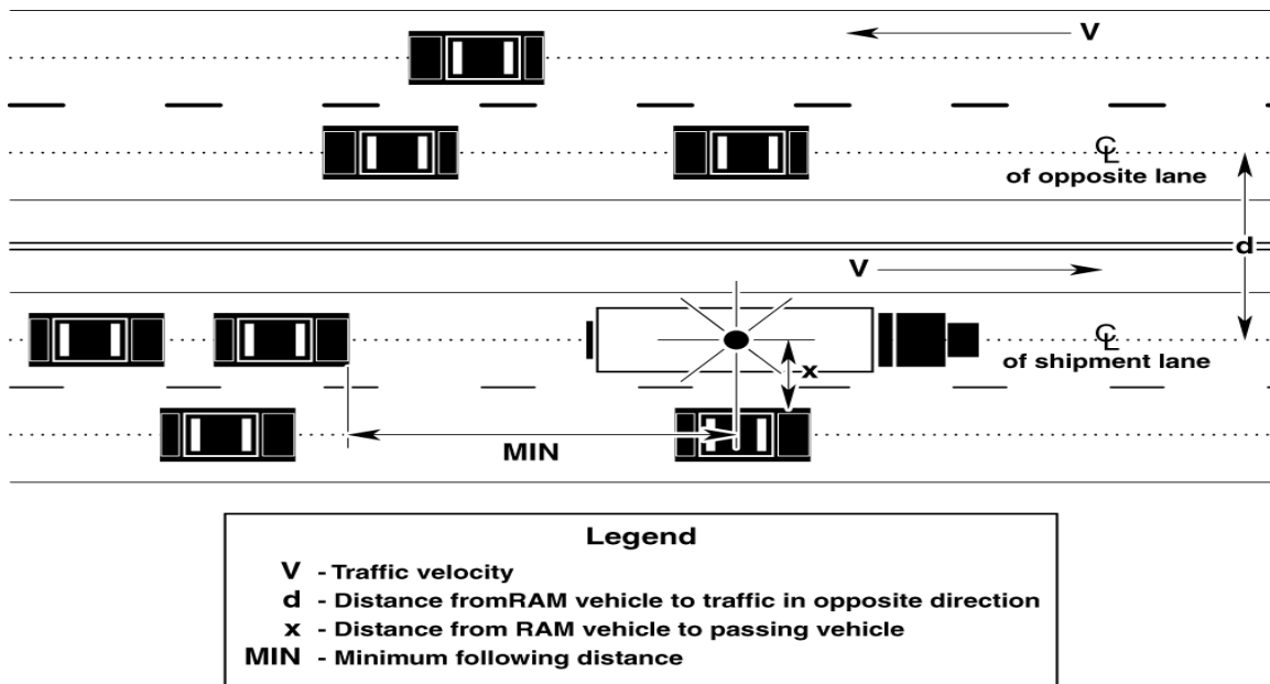
Figure 7. Diagram used in RADTRAN for calculating radiation doses to occupants of other vehicles (from Neuhauser et al., 2000)
