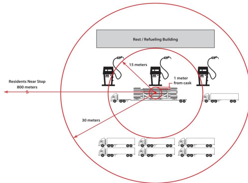
Figure 8. Diagram of truck stop model (not to scale).
