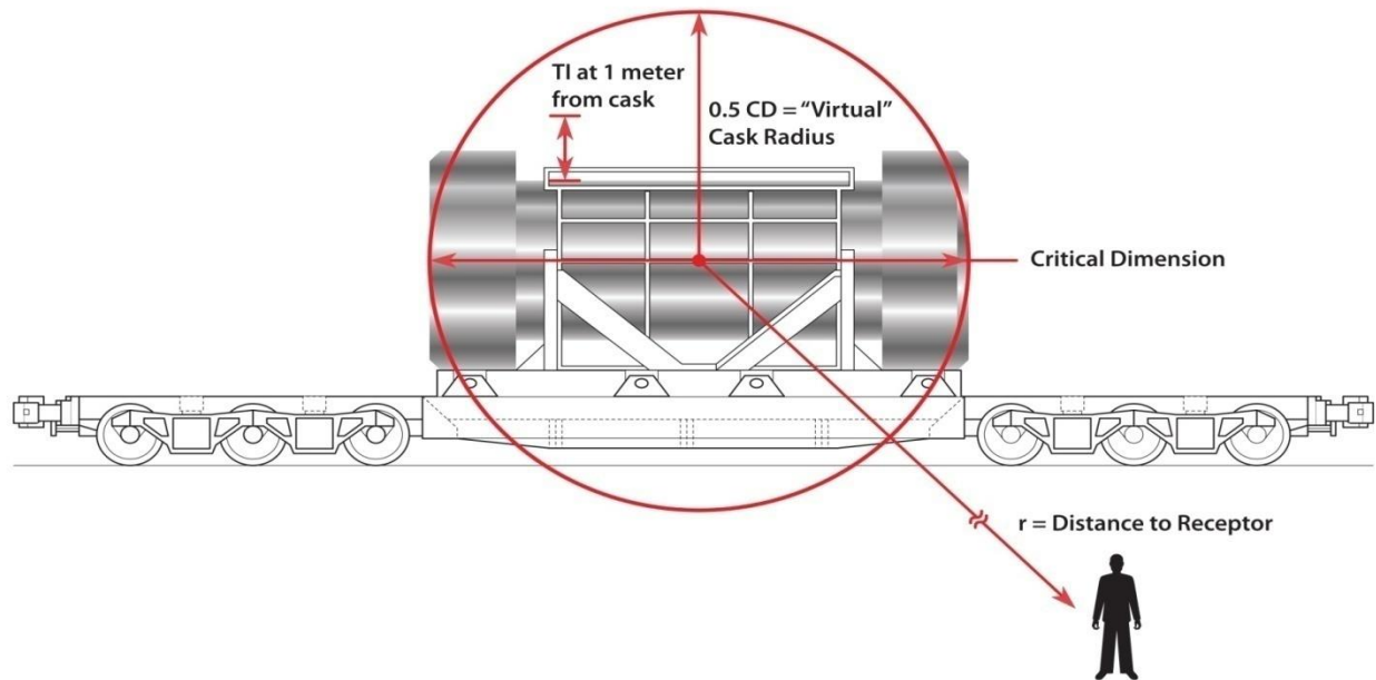
Figure 1. RADTRAN model of the vehicle in routine, incident-free transportation. The cask in this diagram is positioned horizontally; the critical dimension is the cask length.
