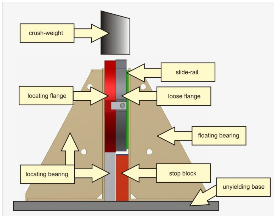
Figure 1. Positioning device with the flange-lid system (sketch)
