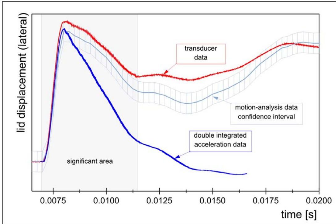
Figure 3. Lid displacement waveforms of different measuring methods
