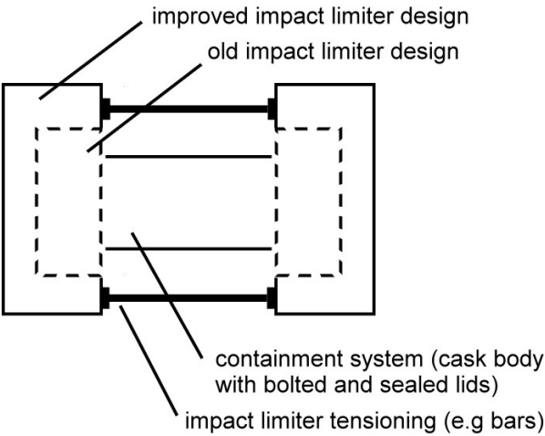
Figure 3. Impact limiter improvement
