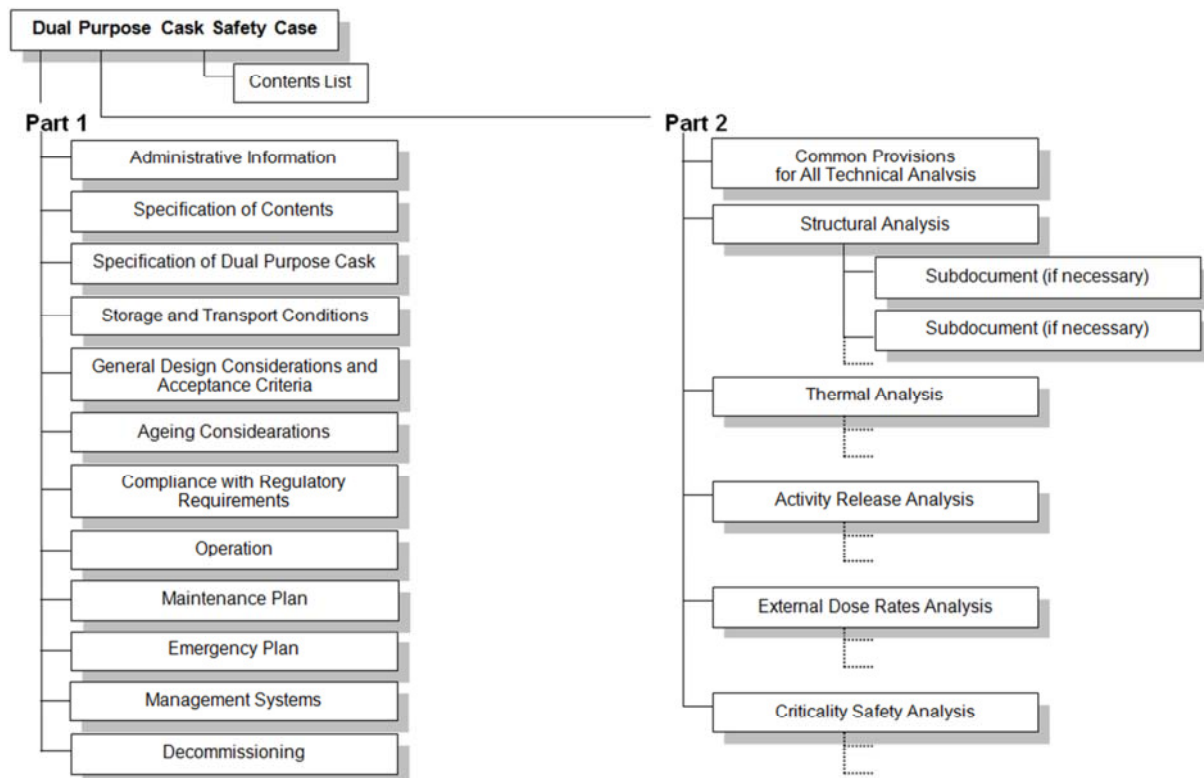
Figure 1. Structure of a PDSR; here for a SNF Dual Purpose Cask [2]
