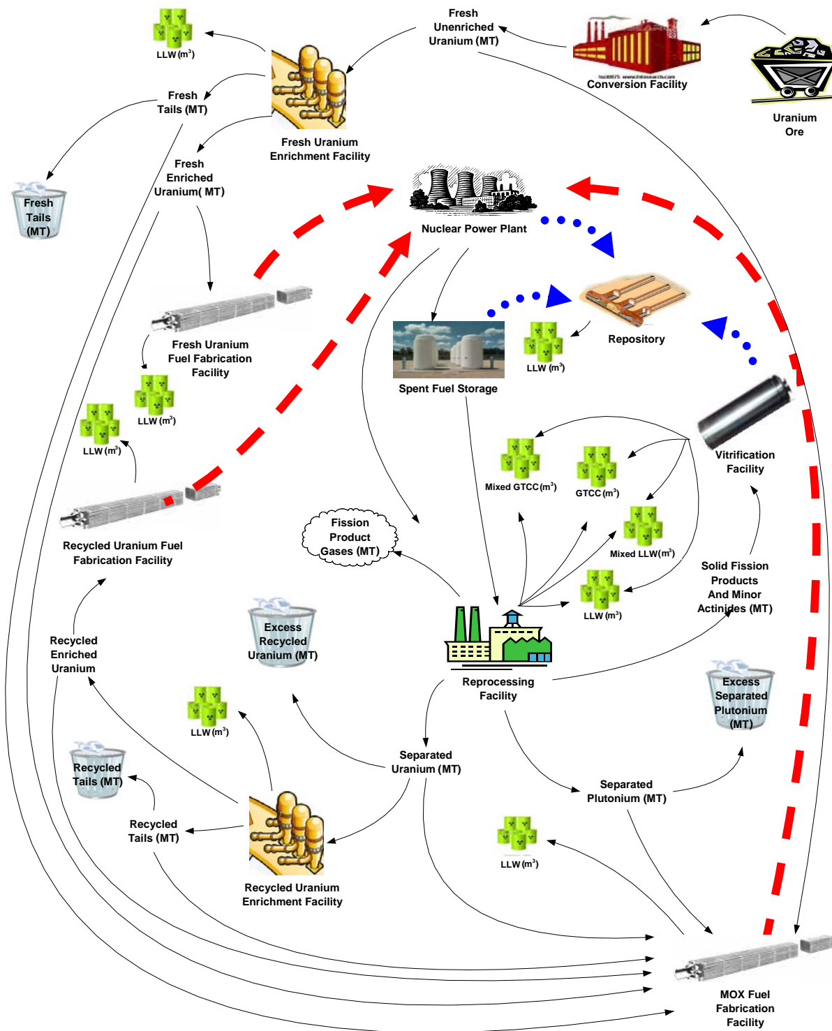
Figure 1. Nuclear Fuel Cycle Process Flow Options
