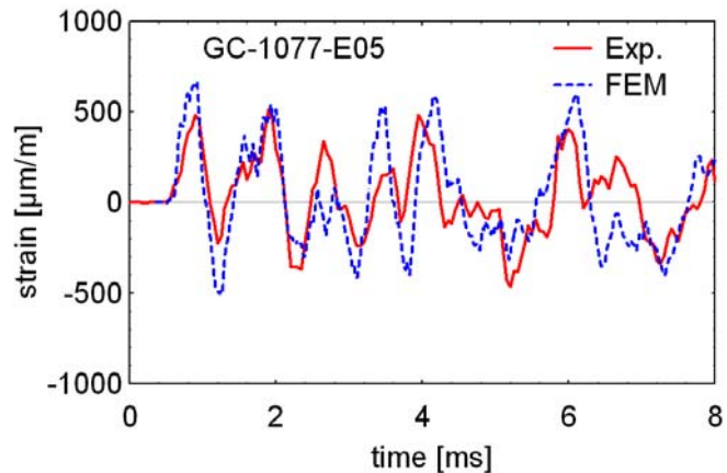
Figure 10. Surface strain in the middle of a side wall of the cubic container during bottom drop from 5.55 m height
