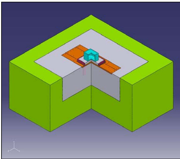
Figure 8. DCI container GC FORM III-2007 with target construction
