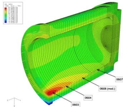
Figure 2. Circumferential strain inside the cylindrical cask for horizontal drop from 0.96 m height
