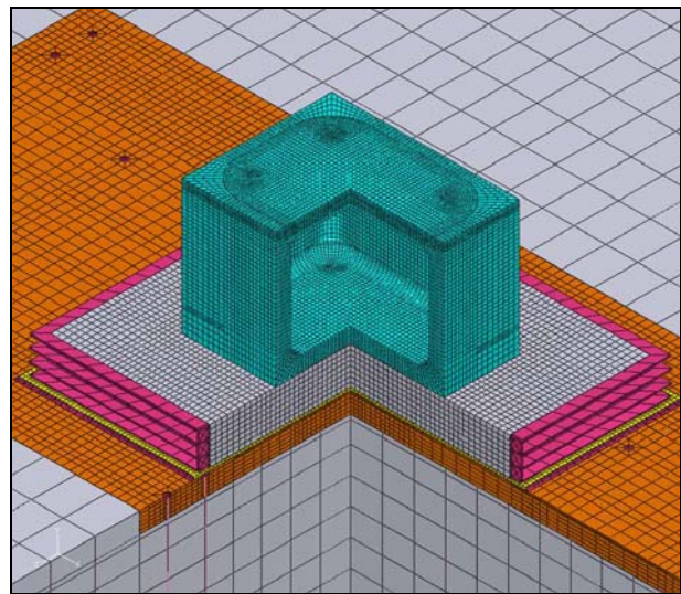
Figure 9. Finite element model acc. to Fig. 8
