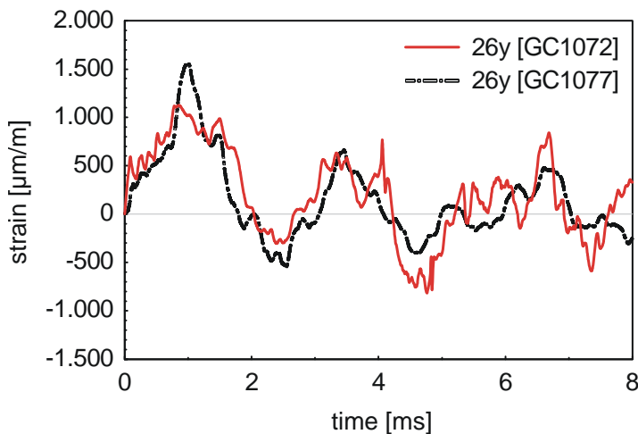
Figure 7. Strain in a fillet at bottom of cubic DCI container before (GC 1072) and after (GC 1077) optimization of target construction
