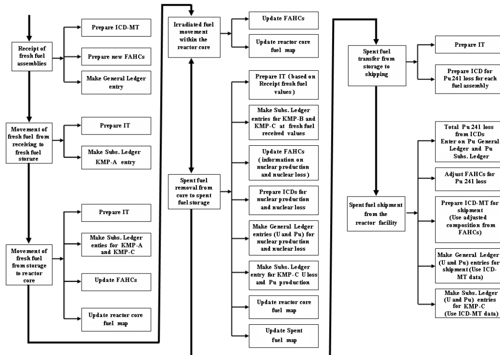
Fig.6. Nuclear material movements and accounting documentation for each (KEMPF et al, 1991)
