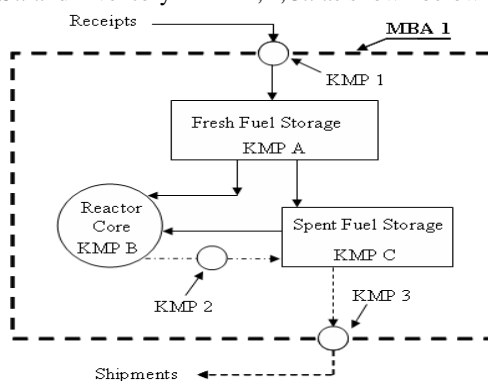
Fig.1. Nuclear material flow sheet in normal operation
