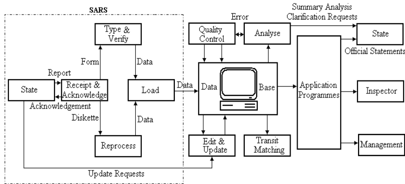
Fig.2. IAEA processing of accounting reports
