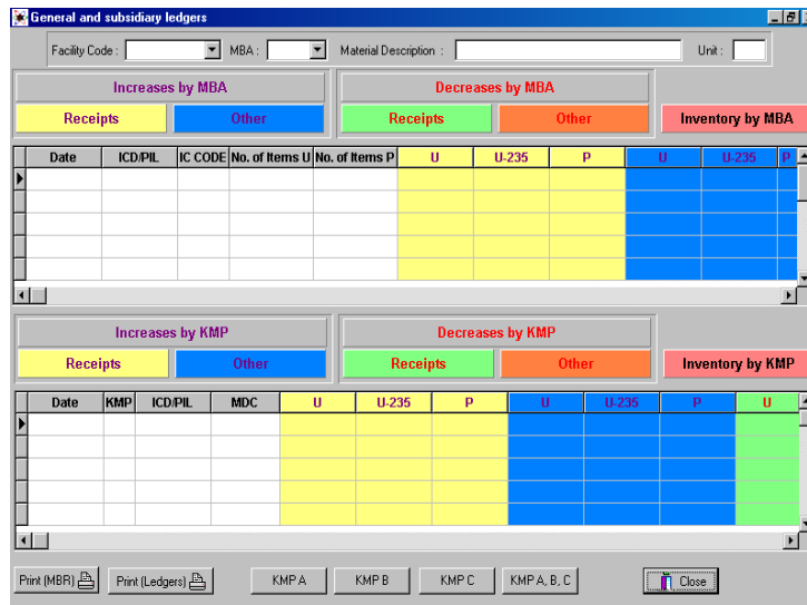
Fig.11. General and subsidiary ledger screen
