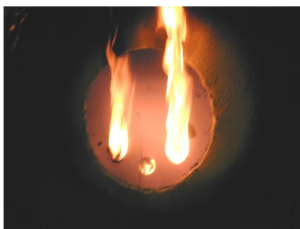
Figure-11 Pail "hotface" immediately after burner removed.
