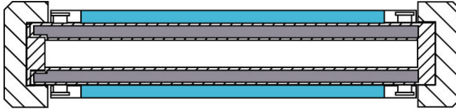
Figure 1. A generic, steel-lead-steel truck cask.
