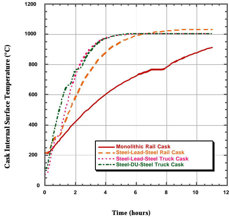
Figure 6, Internal surface temperature histories of the generic casks in an 1000°C long duration fire.
