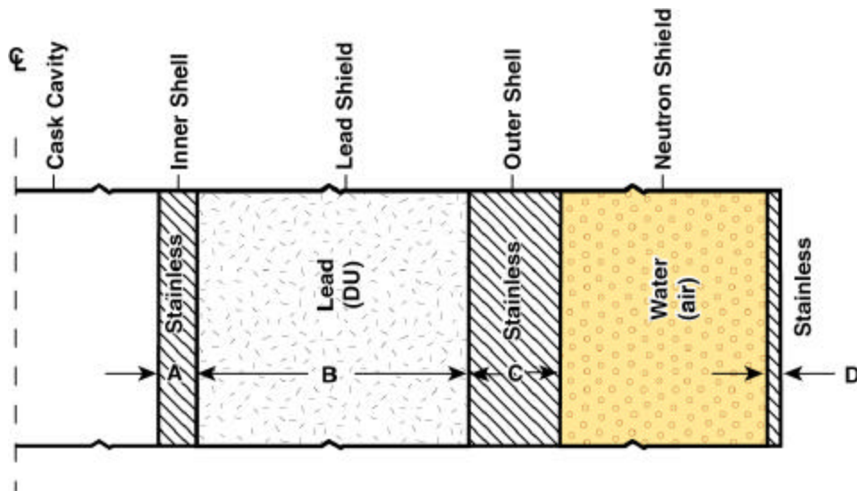
Figure 5. Generic wall cross section used in the 1-D axisymmetric, thermal modeling.
