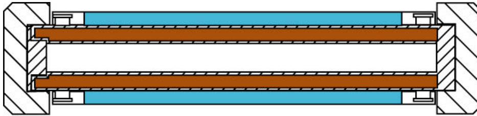
Figure 2. A generic, steel-DU-steel truck cask.
