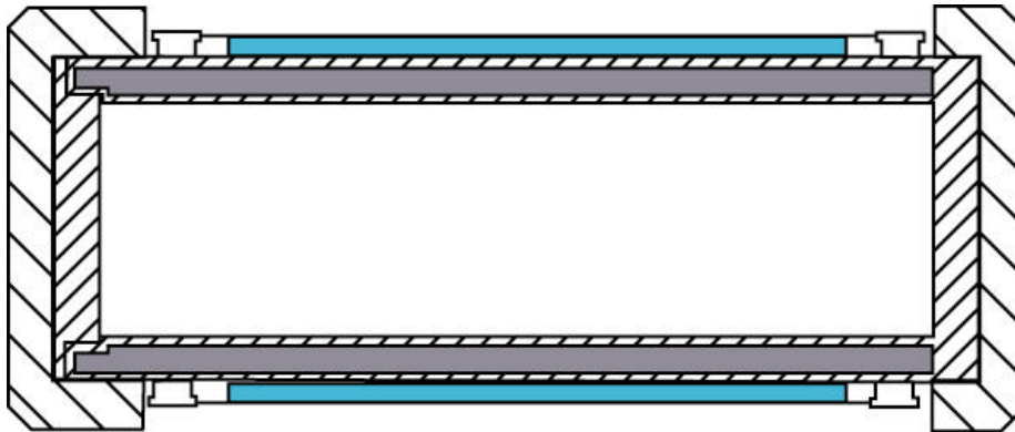
Figure 3. A generic, steel-lead-steel rail cask.
