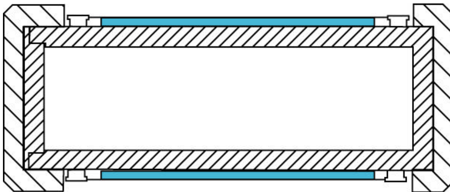
Figure 4. A generic, monolithic steel rail cask.
