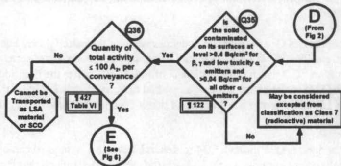
Fig. 5. Logic-flow for initiating screening of objects as SCOs.
