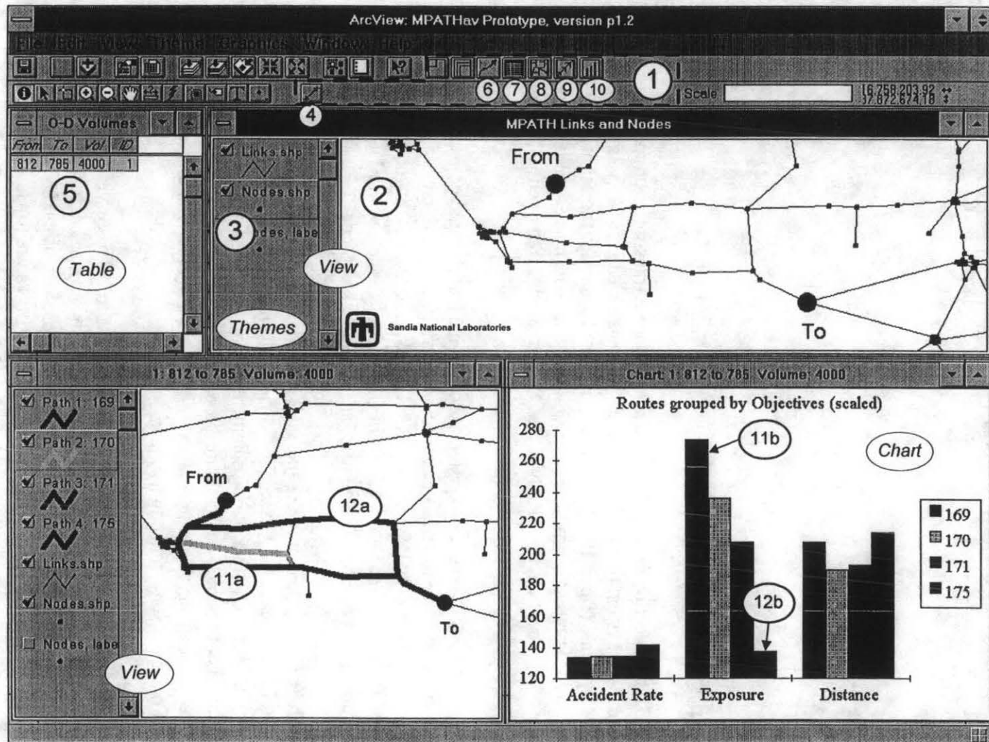
Figure 4 The MPAHav multiobjective routing prototype. See text for explanation of labels.
